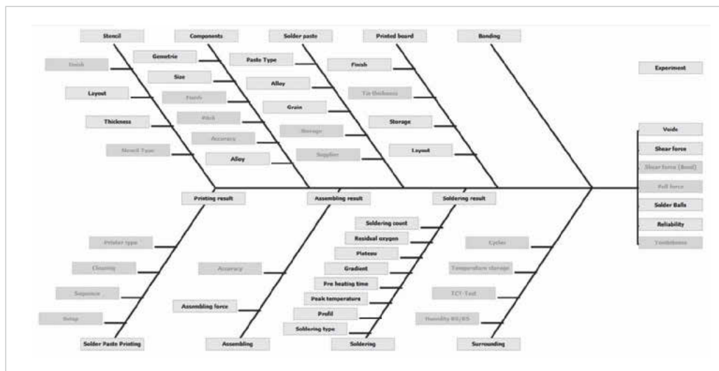
Factors influencing voids and reliability.
