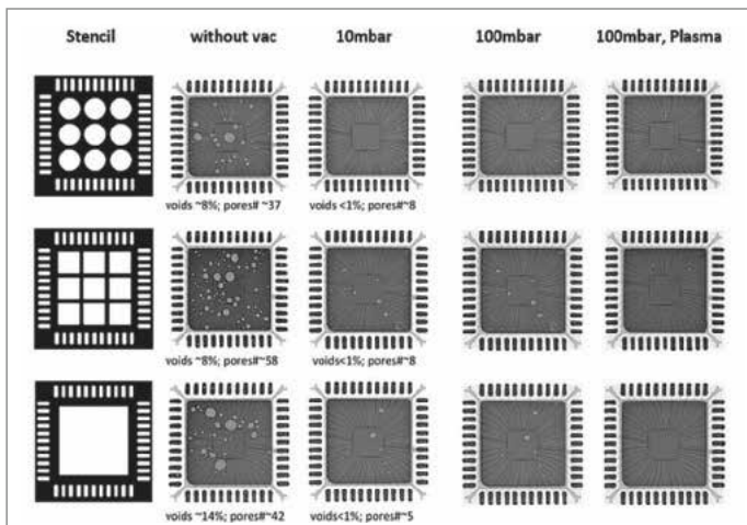
Influencing factor template geometry and template finish.
