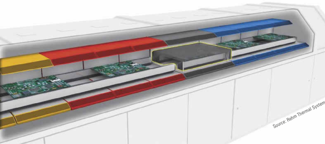
Design of a convection soldering machine with vacuum chamber.
