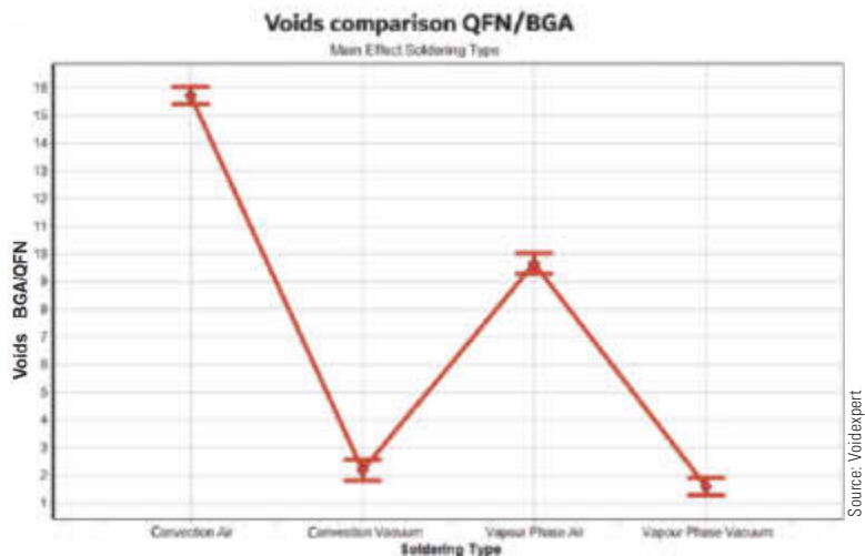
Comparison of the percentage void contents for BGA and QFN components in relation to the soldering process.
