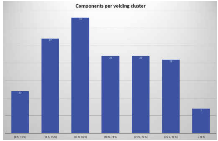
Histogram of surface soldering without vacuum in relation to the void content.
