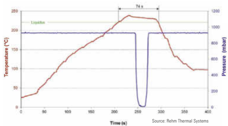
Assembly profile on a convection soldering machine with vacuum process.
